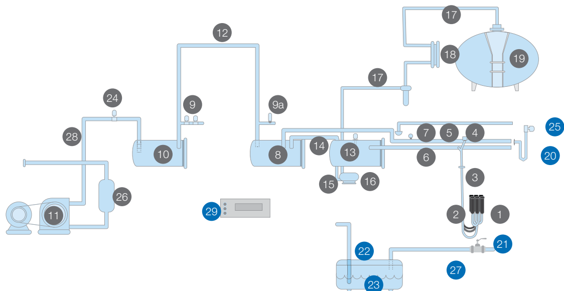
Figure 3 Milking machine schematic
