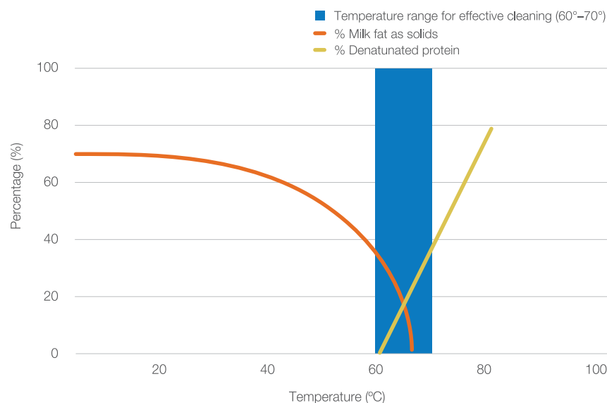
Figure 24 Temperature range for effective cleaning
