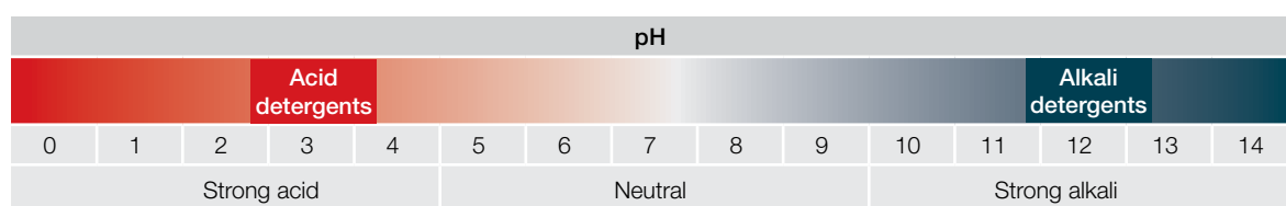
Figure 26 The pH scale showing the required range for acid-based and alkali-based dairy detergents
