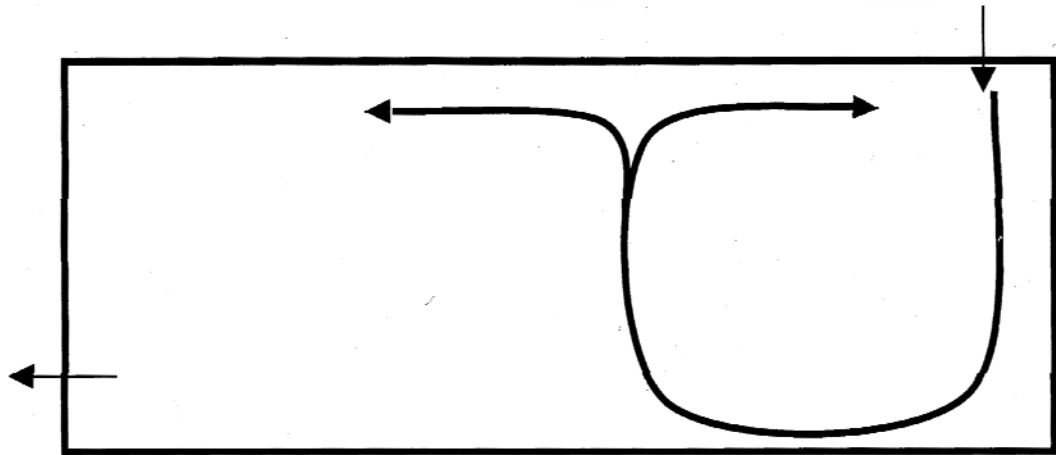
Figure 3. Circulatory currents in ponds with a length-to-width ratio of 3 or more (Shilton and Harrison 2003).
